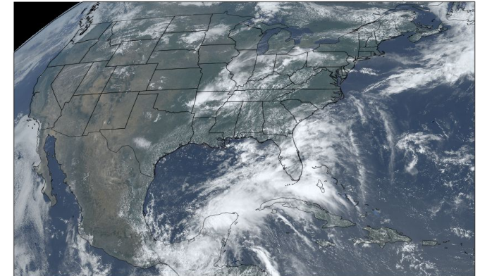
GOES-16 True Color 04 June 2020 16:01 UTC
