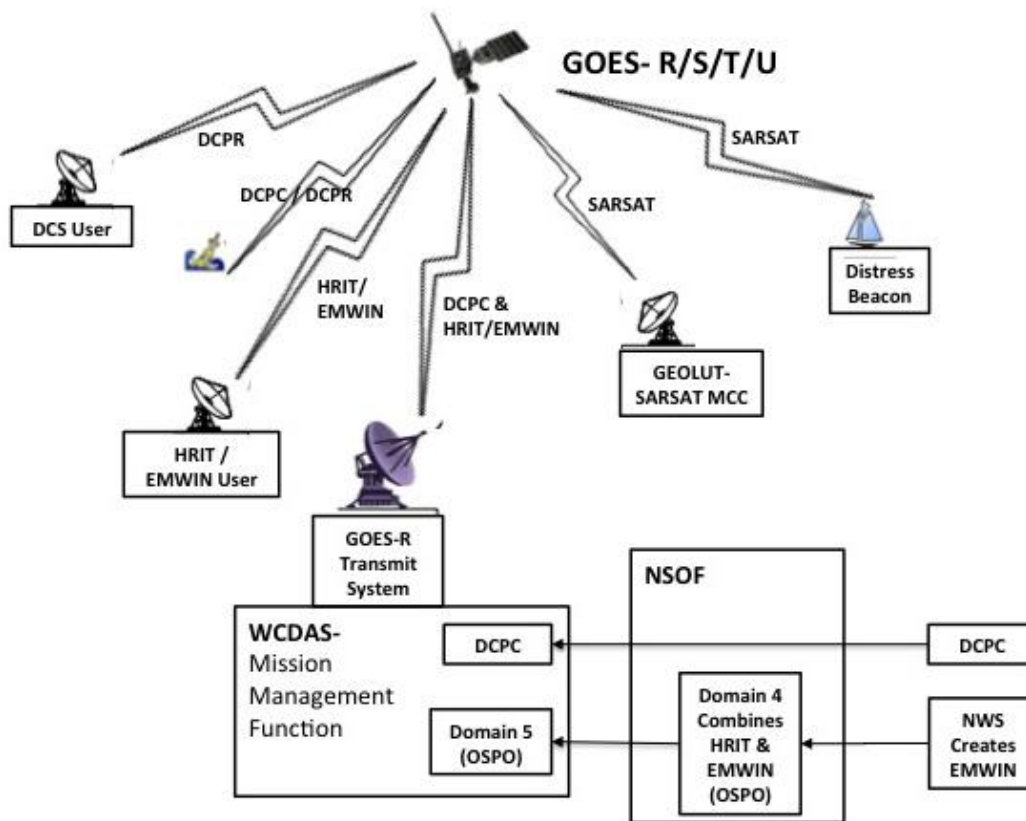
Figure 7: GOES-R Auxiliary Communications Data Distribution System (CCR 1803, CCR 2680A)
